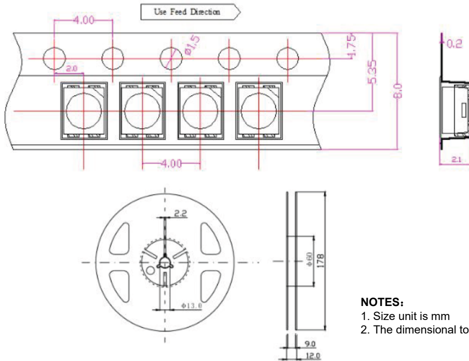
Belt and disk dimensions
