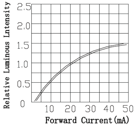
Forward Current VS. Relative Intensity
