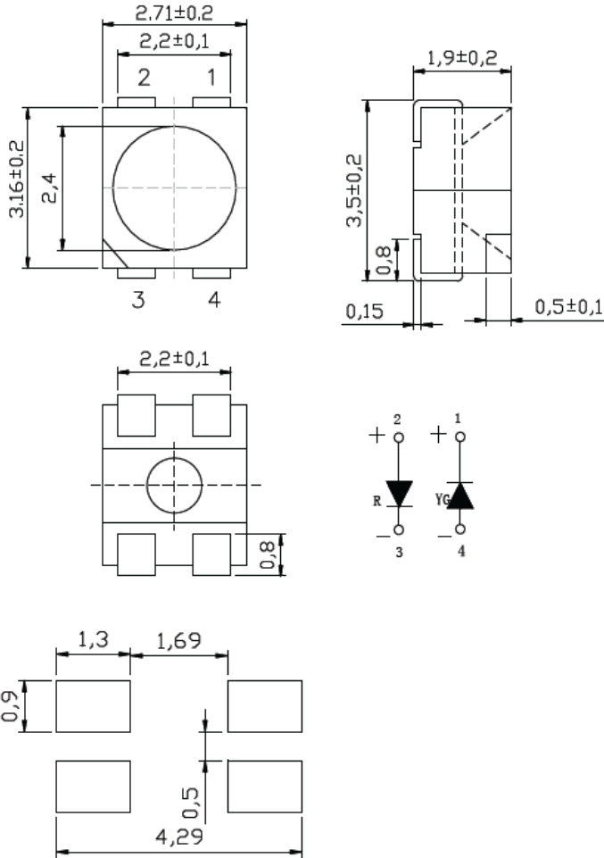
Recommended Soldering Patter
