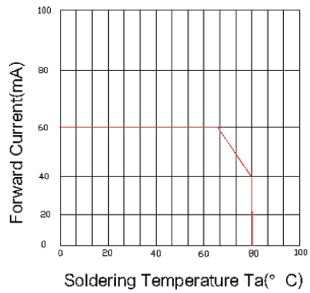
Soldering Temperature VS.Forward Current
