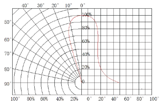
Radiation diagram
