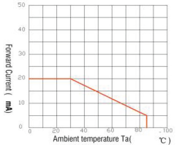
Fig.2 Forward current derating curve Vs. Ambient temperature
