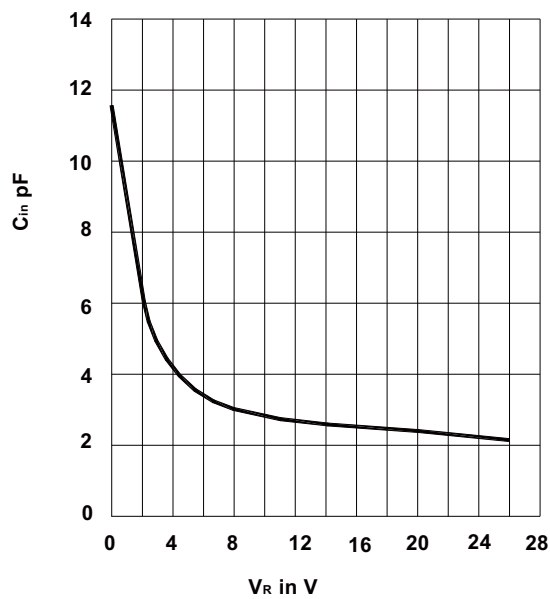
Typical Capacitance o C vs. Reverse Applied Voltage V R
